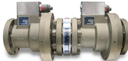
8654 Series Quick Shutoff Valve Double Block & Bleed
