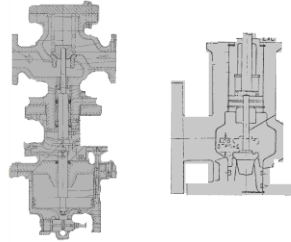
Gas Control and Stop Valves
