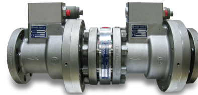
8654 Series Quick Shutoff Valve Double Block & Bleed
