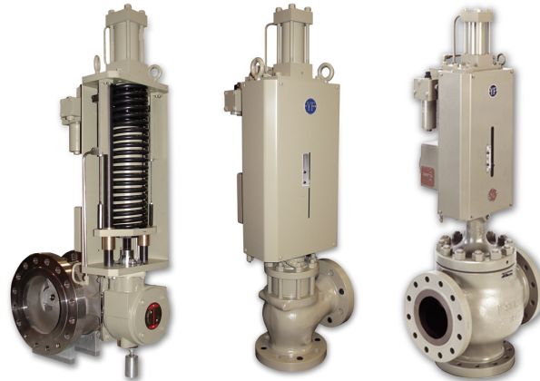
8580 Series Stop/Ratio, Gas Control, and Splitter/Transfer Valves
